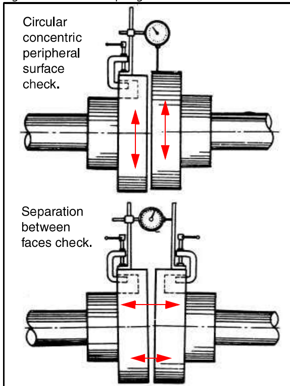
Figure 3. Direct Coupling Checks.
