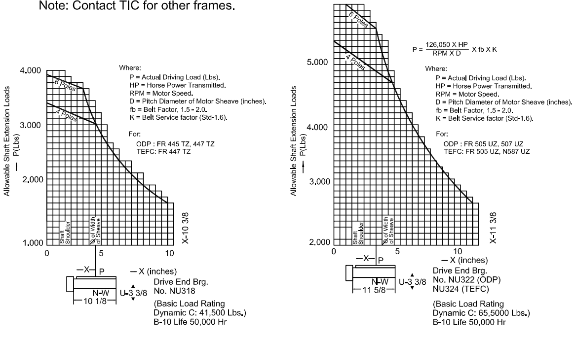
Figure 4. Shaft Extension Loads Due to Transmission of Power.
