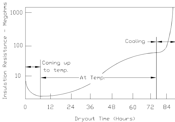
Figure 5. Insulation Resistance vs. Drying Time.
